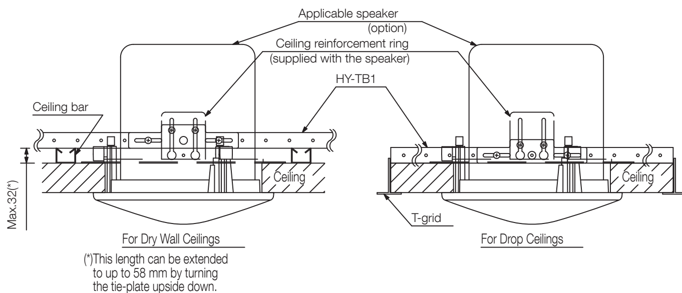
Mounting example
