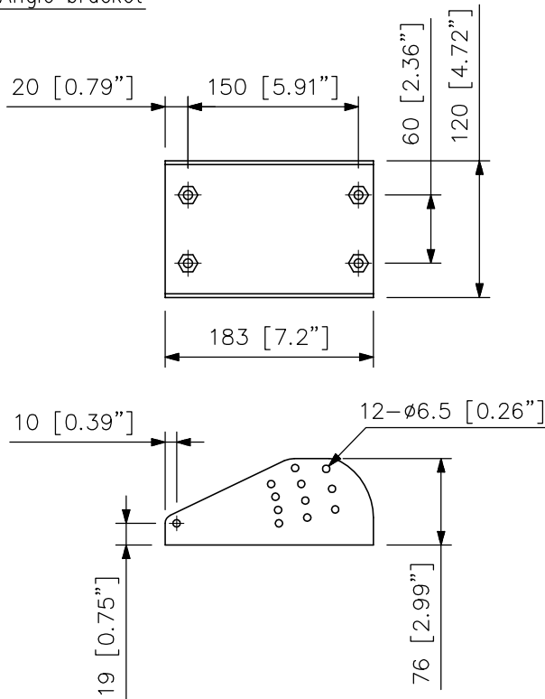
Angle bracket
