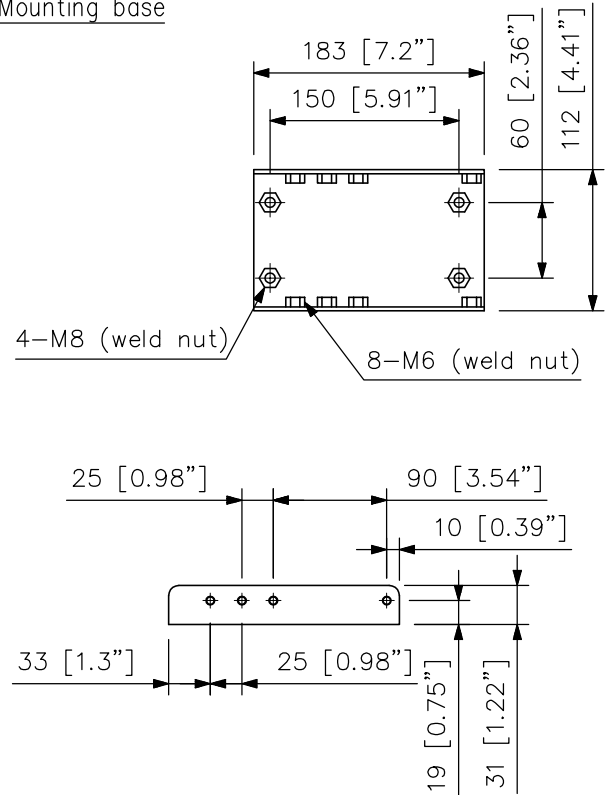
Mounting base
