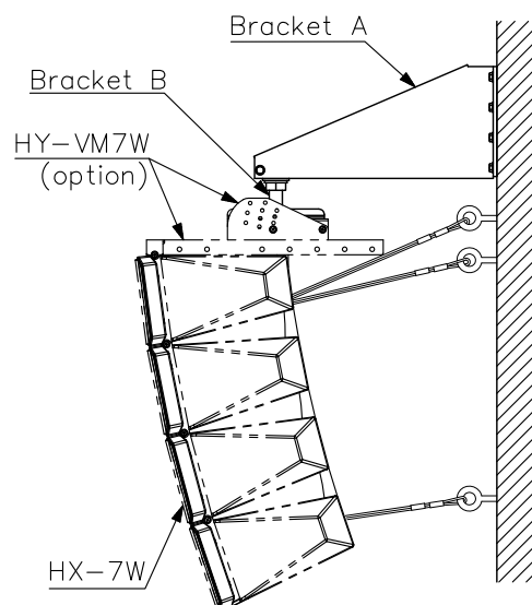
Speaker: 15° mode Bracket: When set to a tilt angle of 0°
